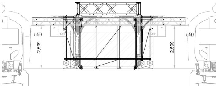
PHASE 3: ENCAPSULATED BLAST AREA SCAFFOLD REMOVED.
