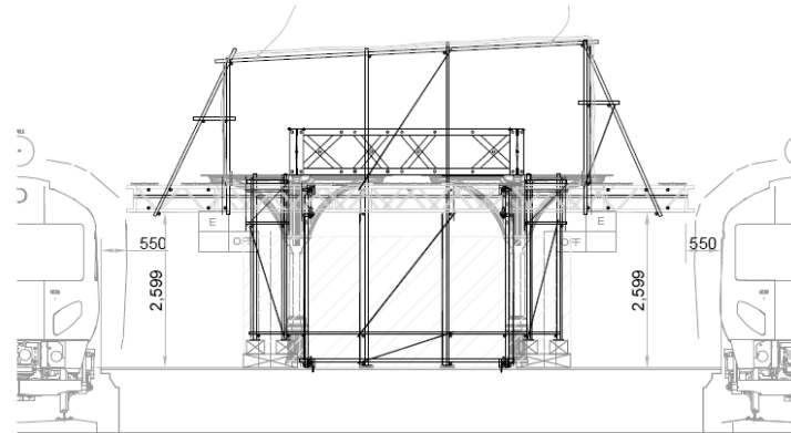
PHASE 2: ERECT ENCAPSULATED BLAST AREA SCAFFOLD.
