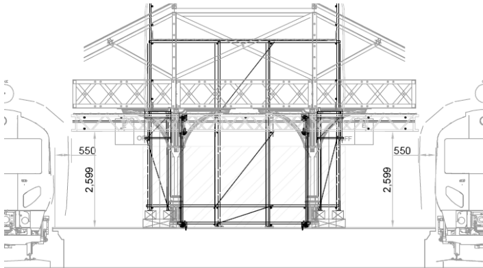
PHASE 1: ERECT CANOPY DEMOLITION SCAFFOLD
