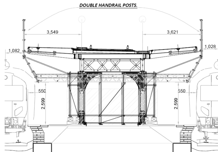
PHASE 4: NEW STEELWORK CONSTRUCTION
